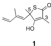
Figure 1. Structure of thiolactomycin.
