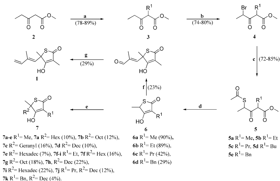
Scheme 1. Reagents and conditions: (a) \text{R}^1\text{X} , \text{K}_2\text{CO}_3 (4 equiv), THF, reflux; (b) \text{PyBr}_3 , \text{AcOH} , rt; (c) \text{AcSH} , \text{Et}_3\text{N} , \text{EtOAc} , rt; (d) \text{KOH} (2 equiv), \text{H}_2\text{O}/\text{EtOH} (1:1), 45^\circ\text{C} ; (e) \text{NaH} (1.2 equiv), \text{BuLi} (1.1 equiv), \text{R}^2\text{X} , THF/DMPU (1:1), rt to -78^\circ\text{C} ; (f) \text{NaH} , \text{BuLi} , \text{C}_2\text{H}_5\text{OCHC}(\text{CH}_3)\text{CHO} (2 equiv), THF/Pyrimidone (1:1), rt to -78^\circ\text{C} ; (g) \text{BuLi} (2 equiv), \text{Ph}_3\text{P}^+-\text{CH}_3\text{Br}^- , THF, -78^\circ\text{C} to rt.
